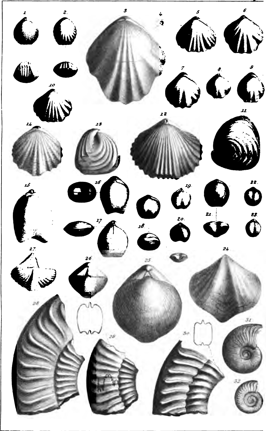
Gunstedt, Jura.
